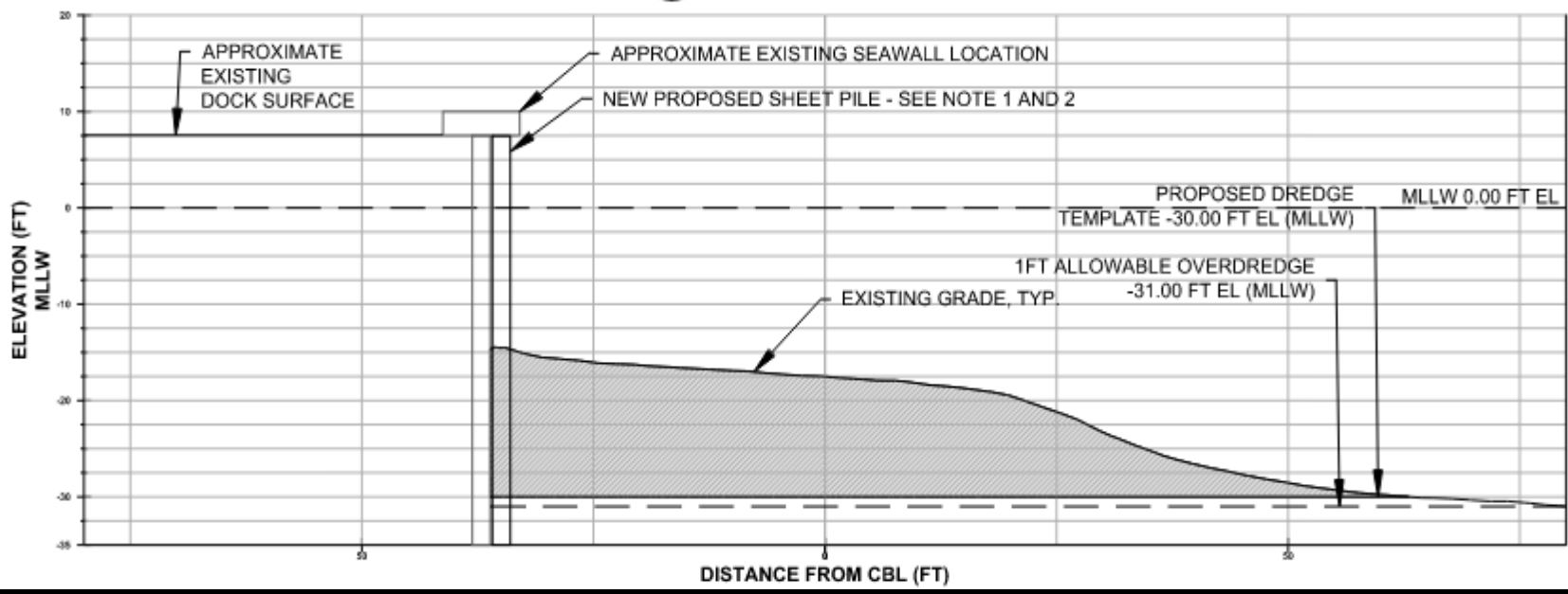
A C-102 TYPICAL CUT- PROPOSED DREDGE AREA DREDGE TEMPLATE PROFILE
