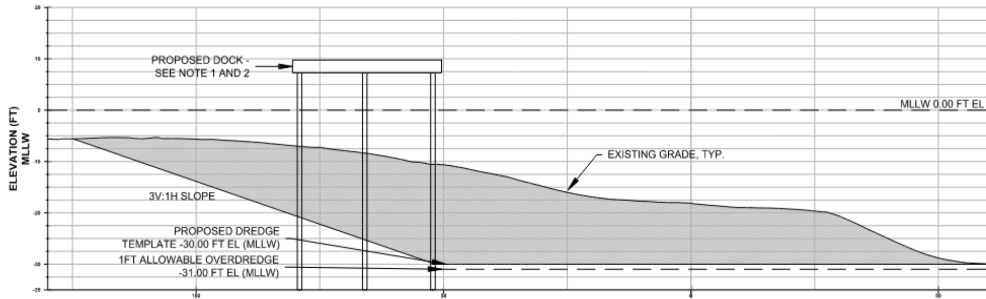
A C-102 TYPICAL CUT- PROPOSED DREDGE AREA DREDGE TEMPLATE PROFILE
