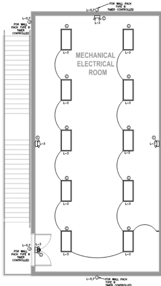
MEP STAND LIGHTING FLOOR PLAN
