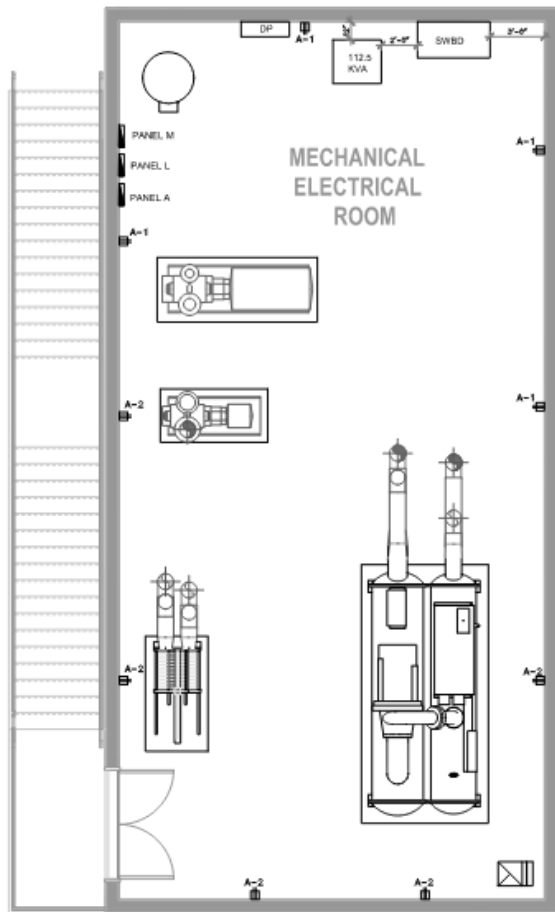
MEP STAND POWER FLOOR PLAN
